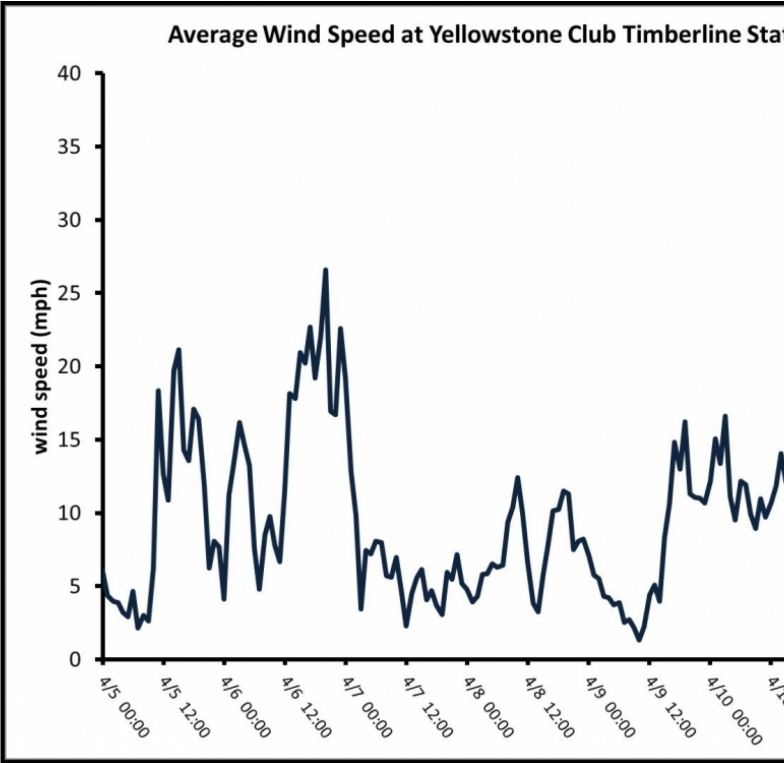
Average winds from the Timberline station at the Yellowstone Club at 9800 feet.
