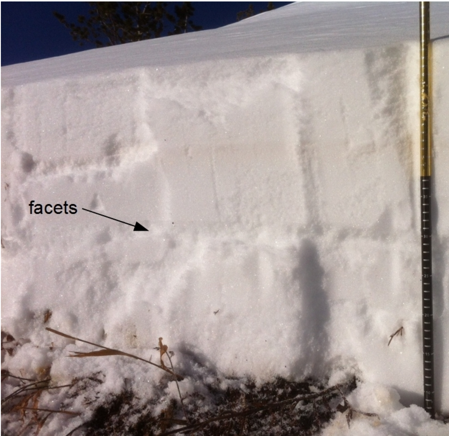
The snowpack in Beehive Basin north of Big Sky is generally 2-3 feet deep. An obvious layer of facets can be found in most places in the lower half of the snowpack. The latest snowfall, 3 days ago, does not seem to have stressed this layer enough to create unstable conditions. Finding this layer and doing a stability test or two only takes a few minutes. Photo: C. Diaz
